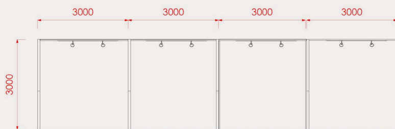
FRONT VIEW
